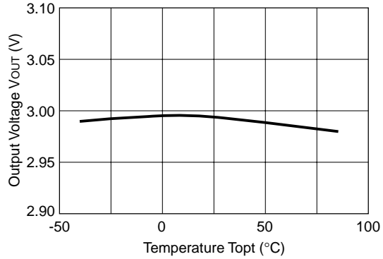
Regulator3 (3V)
