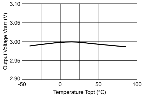
Regulator5 (3V)
