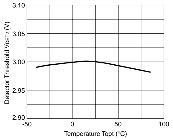
Detector2 (3.0V)
