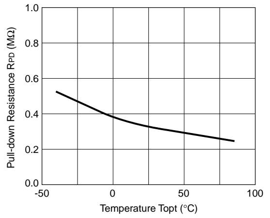
Pull-down Resistance
