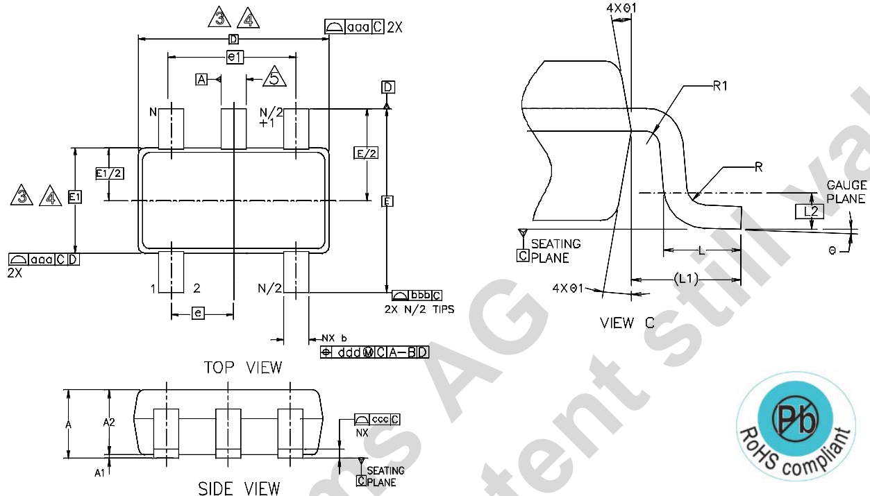
Figure 22. TSOT23-5 Package
