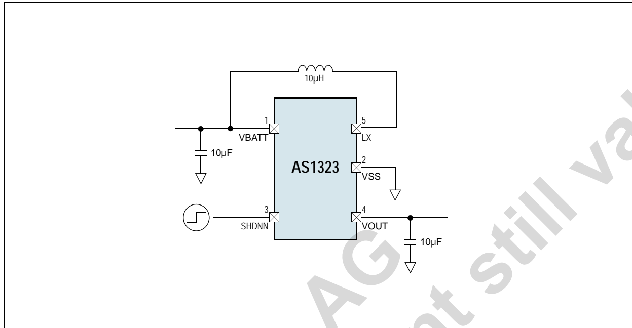
Figure 21. Typical Application
