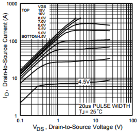
Fig. 1 Typical Output Characteristics, T_C = 25^{\circ}
