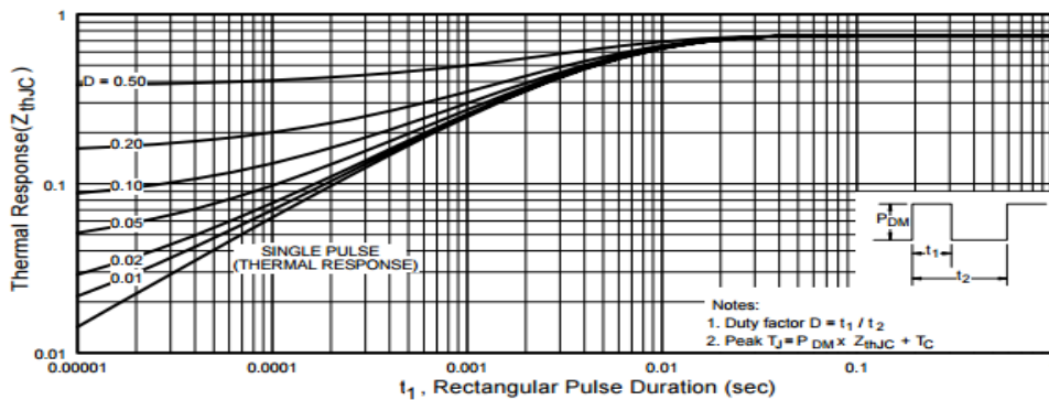
Fig. 9 - Maximum Effective Transient Thermal Impedance, Junction-to-Case
