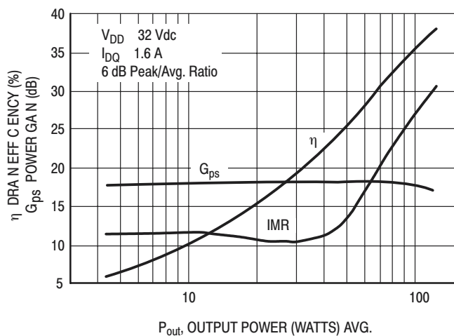
Figure 5. 8-VSB Performance (860 MHz)
