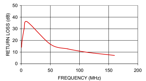
TC16-161T+ INPUT RETURN LOSS
