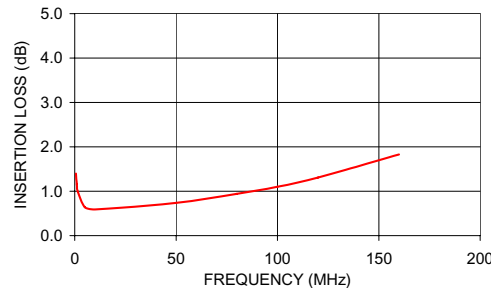
TC16-161T+ INSERTION LOSS
