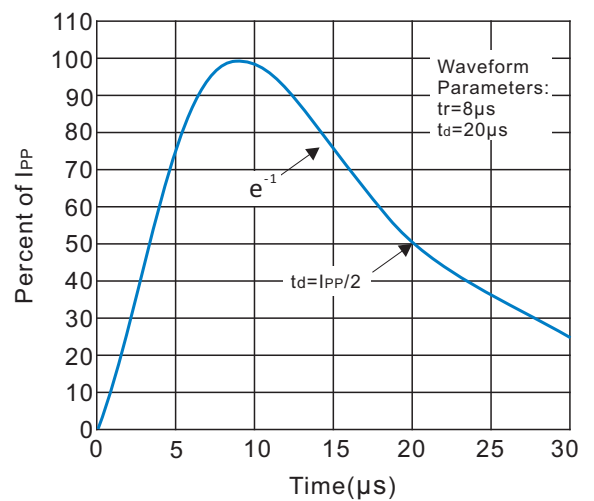
Fig.2 Pulse Waveform
