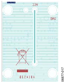
Figure 18. Evaluation Board Layout (Bottom)
