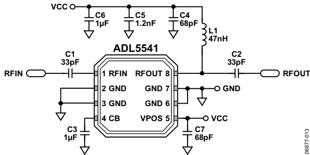
Figure 14. Basic Connections
