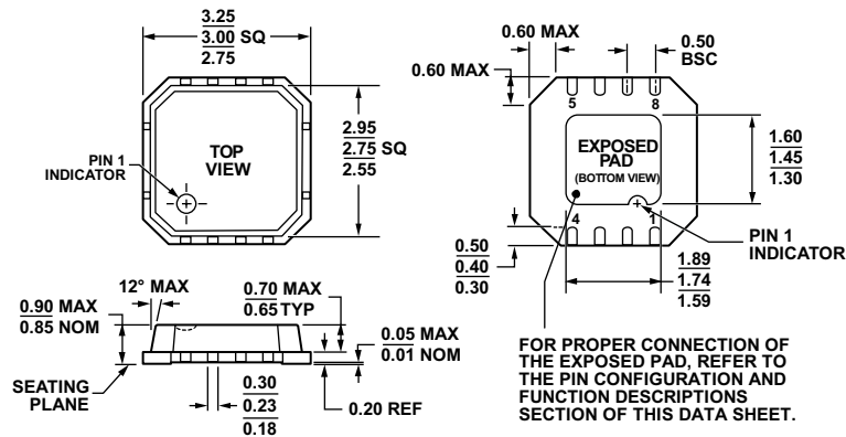
Figure 21. 8-Lead Lead Frame Chip Scale Package [LFCSP_VD] 3 mm x 3 mm Body, Very Thin, Dual Lead (CP-8-2) Dimensions shown in millimeters
