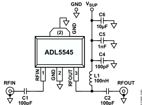
Figure 41. Evaluation Board Schematic
