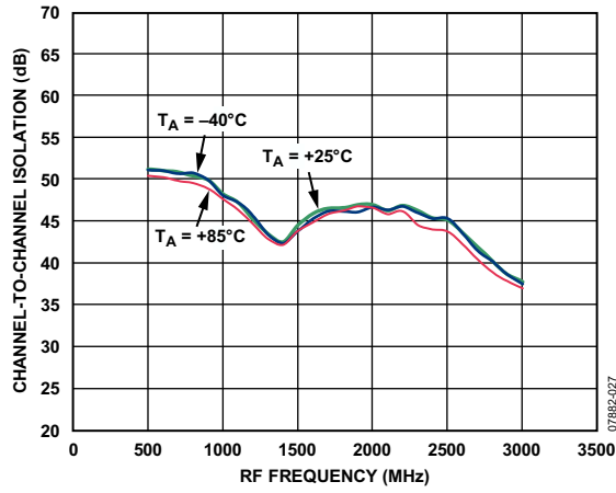
Figure 27. Channel-to-Channel Isolation
