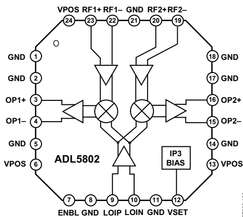
Figure 67. ADL5802 Block Diagram
