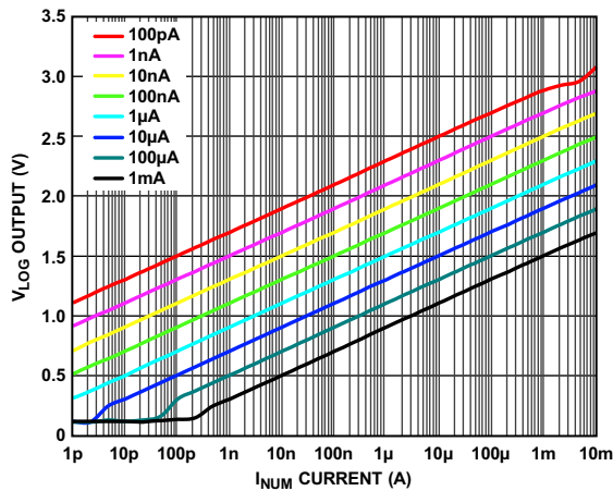
Figure 5. V_{LOG} vs. I_{NUM} for Multiple Values of I_{DEN} (Decade Steps from 100 pA to 1 mA)
