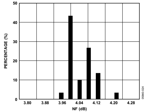
Figure 25. Noise Figure Distribution at 880 MHz
