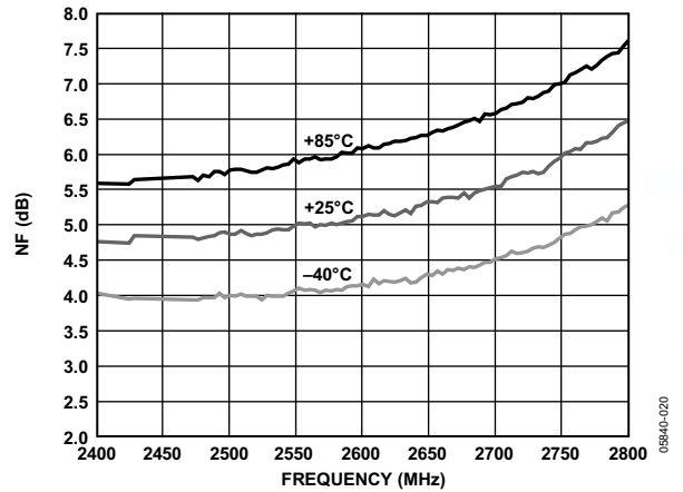
Figure 21. Noise Figure vs. Frequency and Temperature, 2500 MHz to 2700 MHz
