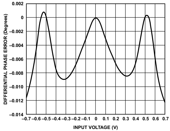
Figure 52. ADV3229 Differential Phase Error
