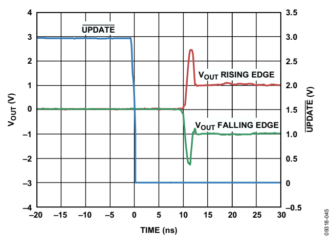
Figure 47. ADV3229 Enable Time
