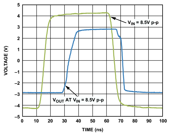
Figure 53. ADV3229 Overdrive Recovery
