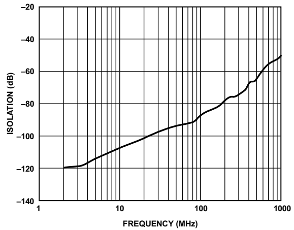
Figure 30. ADV3229 Off Isolation
