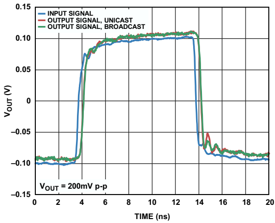
Figure 14. ADV3228 Small Signal Pulse Response
