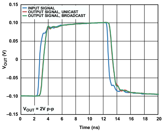
Figure 15. ADV3228 Large Signal Pulse Response
