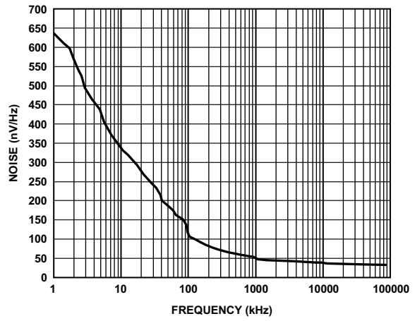
Figure 29. ADV3229 Output Noise, 100 \Omega Load
