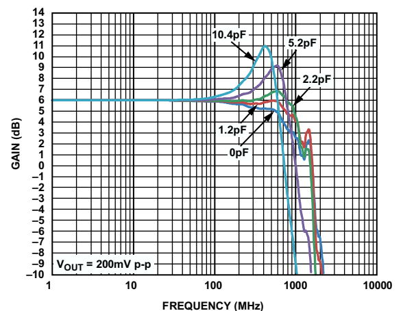
Figure 12. ADV3229 Small Signal Frequency Response, R_L = 150 \Omega
