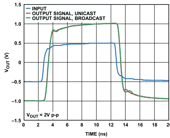
Figure 18. ADV3229 Large Signal Pulse Response
