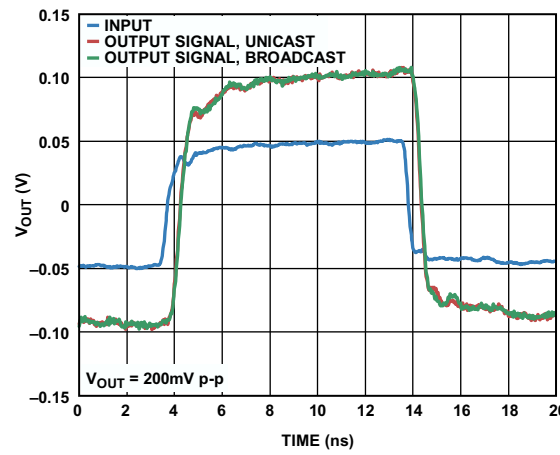
Figure 17. ADV3229 Small Signal Pulse Response
