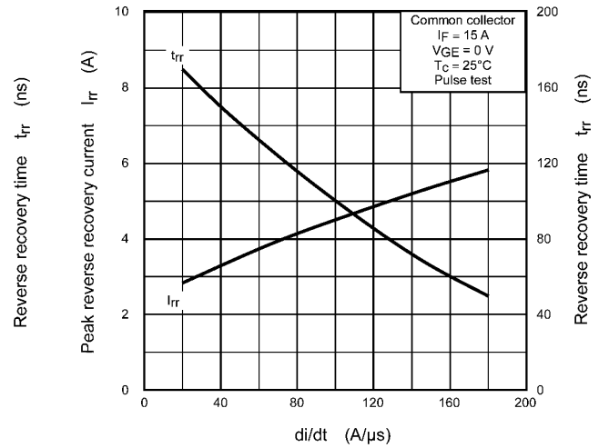
Fig. 8.16 I_{rr}, t_{rr} - di/dt
