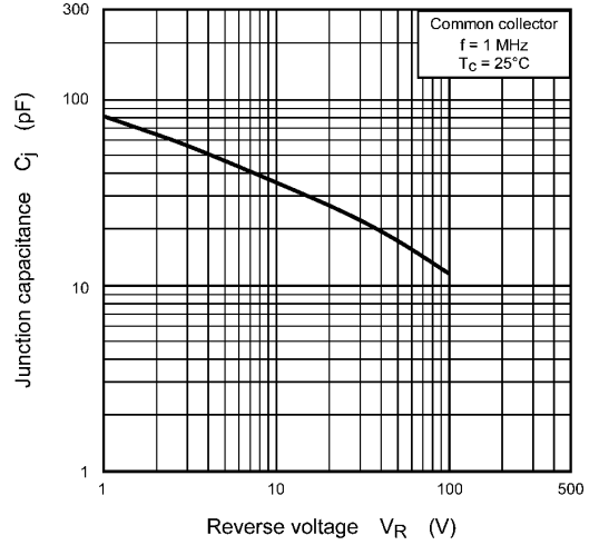
Fig. 8.14 C_j - V_R
