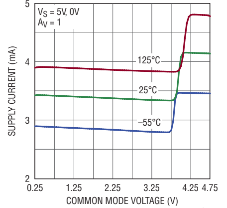
Supply Current vs Input Common Mode Voltage (Per Amplifier)
