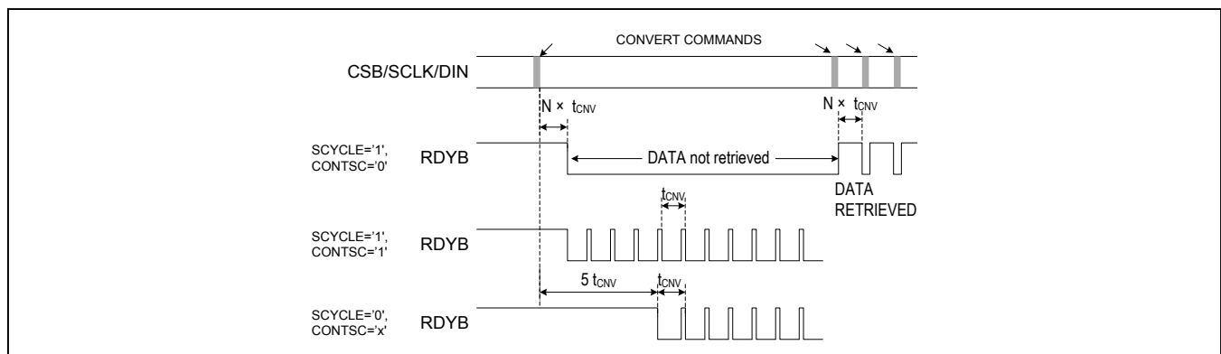
Figure 4. Timing of RDYB in All Conversion Configurations: Single-Cycle, Single-Cycle Continuous, and Continuous. In sequencer mode 1 and in sequencer modes 2 and 3, with SEQ:RDYBEN='0' N = 1 . In sequencer modes 2 and 3 with SEQ:RDYBEN='1' N = number of active channels.
