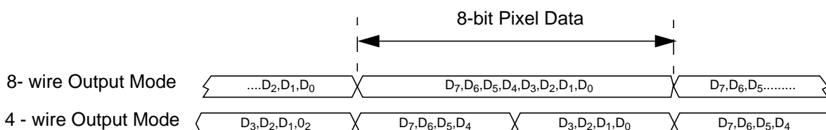
Figure 6 : Output Modes
