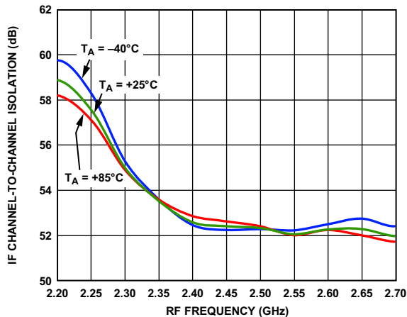
Figure 44. IF Channel-to-Channel Isolation vs. RF Frequency
