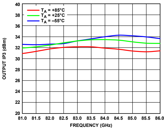
Figure 17. Output IP3 vs. Frequency over Various Temperatures, I_{DD} = 800 \text{ mA} , P_{OUT}/\text{Tone} = 14 \text{ dBm}
