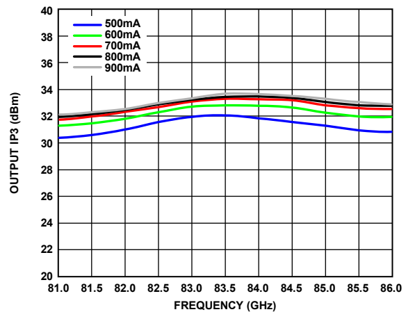
Figure 20. Output IP3 vs. Frequency over I_{DD} , P_{OUT}/\text{Tone} = 14 \text{ dBm}
