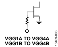
Figure 8. VGG1A to VGG4A and VGG1B to VGG4B Interface Schematic
