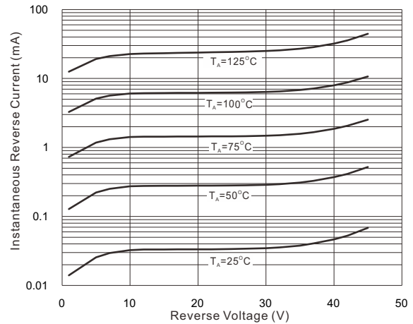
Fig. 2 - Reverse Characteristics
