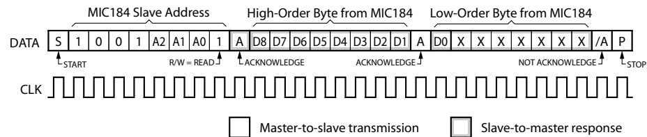
Figure 5. RECEIVE_DATA from a 16-Bit Register
