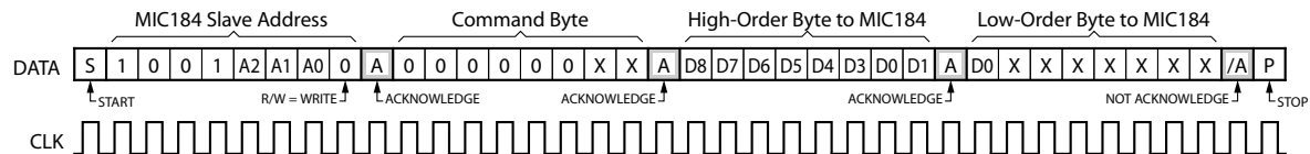
Figure 3. WRITE_WORD Protocol
