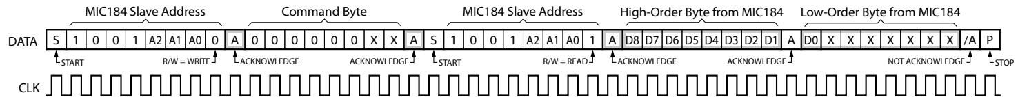
Figure 4. READ_WORD Protocol
