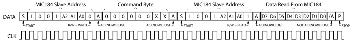
Figure 2. READ_BYTE Protocol
