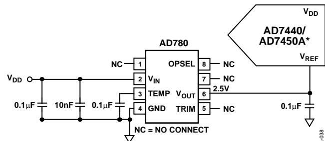
Figure 38. Typical V_{REF} Connection Diagram for V_{DD} = 5 V
