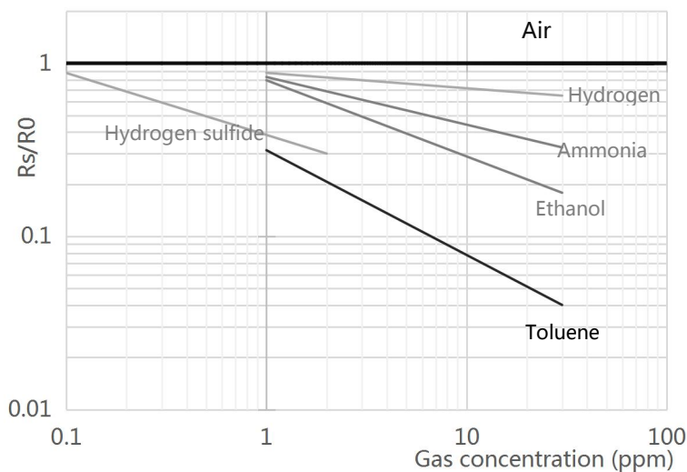
Figure 6 TVOC Sensitivity Characteristics
